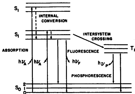
Figure 1.3. Jablonski diagram.
