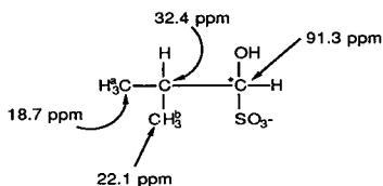
FIGURE 14. 13 C chemical shift data for the 2-methylpropanal bisulfite addition product in D 2 O. Note that bisulfite addition leads to formation of a chiral center and diastereotopic carbons.
