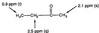
FIGURE 15. ^1\text{H} chemical shift data for an aqueous solution of 2-butanone.
