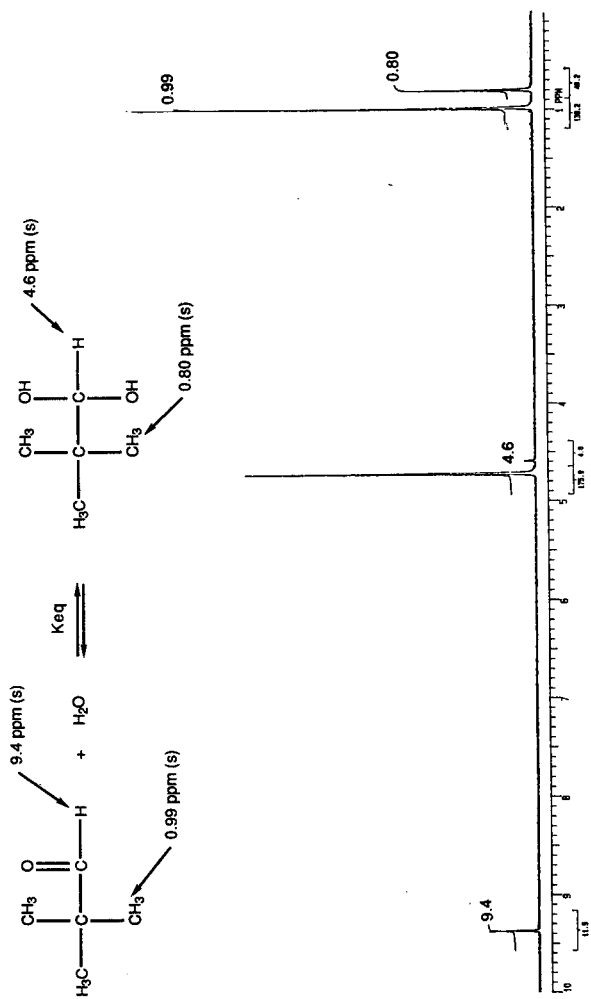
FIGURE 36. ^1H spectrum for the trimethylacetalddehyde-hydrate equilibrium in D_2O .
