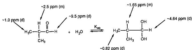
FIGURE 11. ^1\text{H} chemical shift data for the 2-methylpropanal-hydrate equilibrium in \text{D}_2\text{O} .
