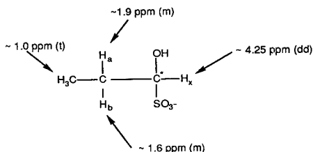
FIGURE 7. 1 H chemical shift data for the propanal bisulfite addition product in D 2 O.
