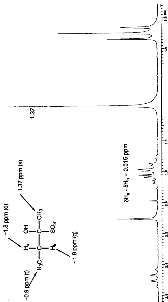
FIGURE 33. ^1\text{H} spectrum for the 2-butanone bisulfite addition product in equilibrium with 2-butanone in D_2O . The methylene hydrogens are split into a doublet of quartets due to the diastereotopism.
