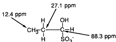
FIGURE 10. ^{13}\text{C} chemical shift data for the propanal bisulfite addition product in \text{D}_2\text{O} .
