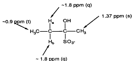
FIGURE 16. ^1\text{H} chemical shift data for the 2-butanone bisulfite addition product in \text{D}_2\text{O} .
