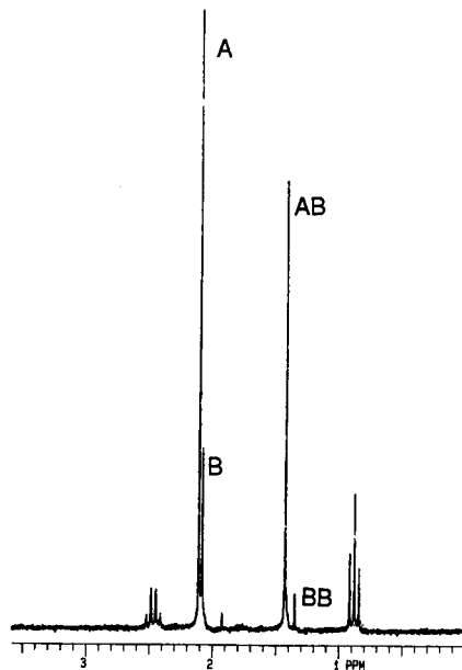
FIGURE 40. ^1\text{H} spectrum obtained from the competition experiment between 0.019M acetone, 0.019M 2-butanone and 0.0096M \text{NaHSO}_3 in \text{D}_2\text{O} .
