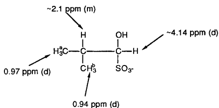
FIGURE 12. 1 H chemical shift data for the 2-methylpropanal bisulfite addition product in D 2 O. \delta\text{H}^a - \delta\text{H}^b = 0.03 ppm.
