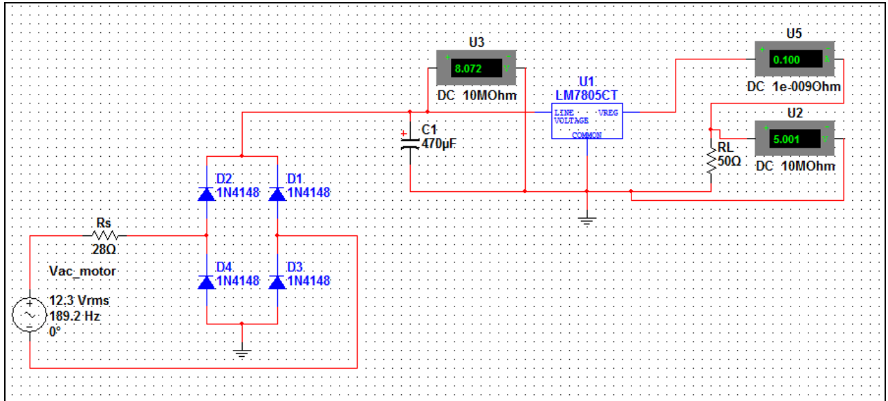
Figure 30 – Multisim simulation of AC generator charging circuit
