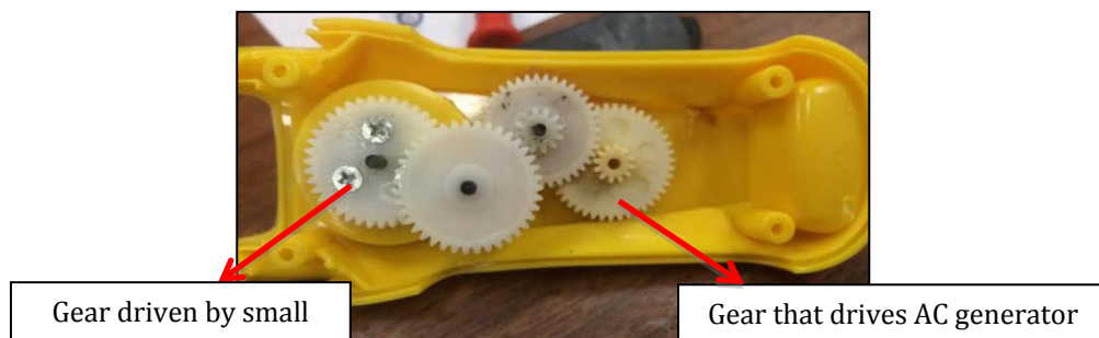
Figure 35 – Gear train in hand crank flashlight
